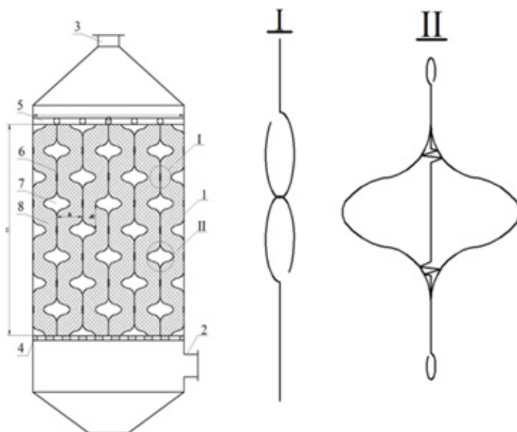
1 – housing; 2,3 - fittings for input and output of purified gas or for output and input of regeneration gas, respectively; 4,5 - support grids; 6 – wires with the help of which bodies of rotation are connected to each other vertically, also between the upper support grid and lower support grid; 7 - bodies of revolution with sharp vertices up and down; 8 – adsorbent.
