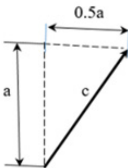
Figure 2. Gas trajectory
